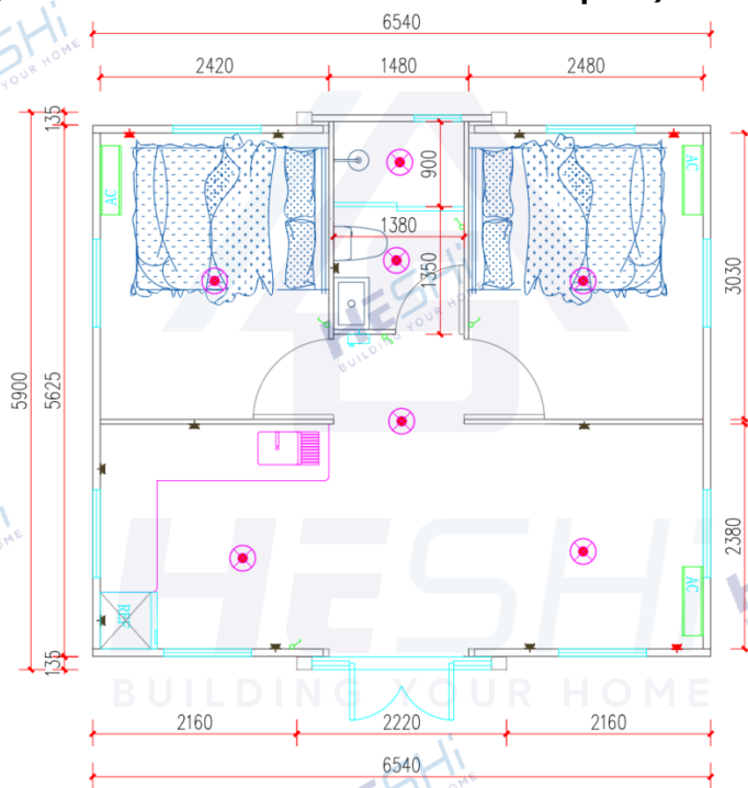
Ground floor plan /SIDE-20FT
