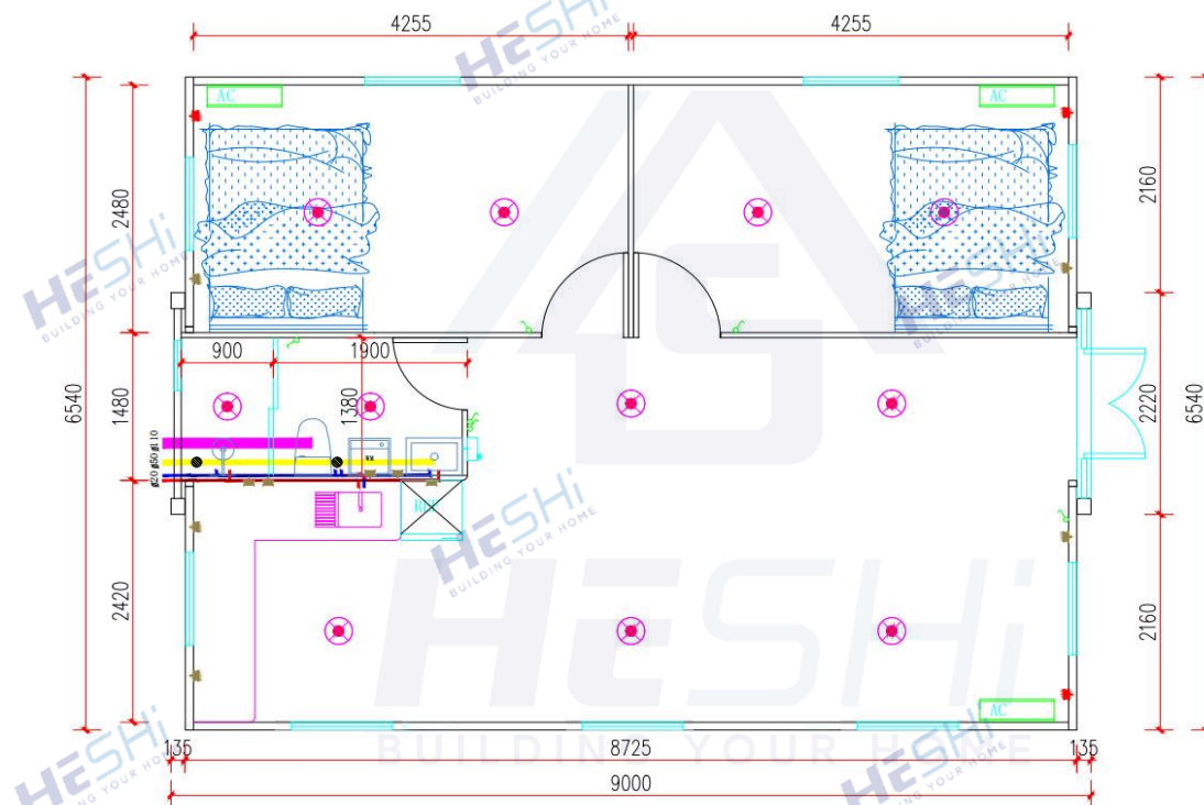
Ground floor plan /SIDE-30FT
