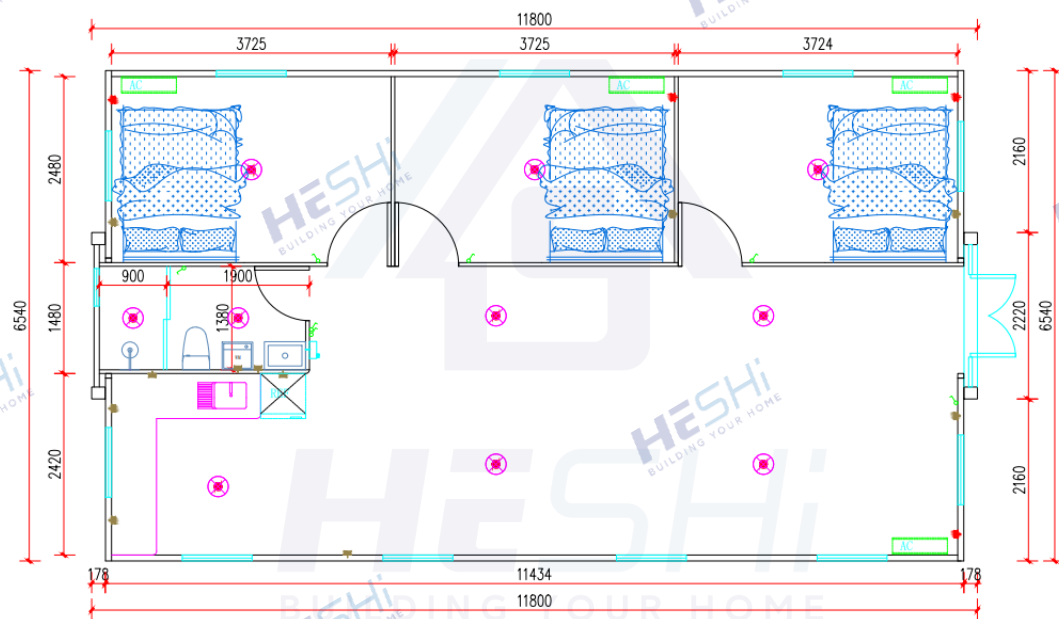
Ground floor plan /SIDE--40FT
