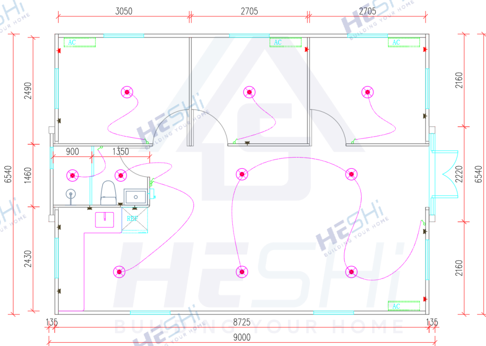
Ground floor plan /SIDE-30FT
